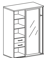
KSK-5 1200x600x2060
