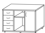
A.МТ-2** 1200x450x670
